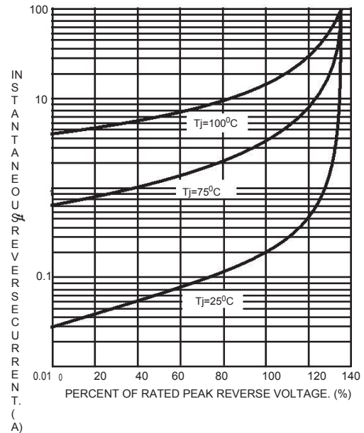
FIG.2- TYPICAL REVERSE CHARACTERISTICS PER BRIDGE ELEMENT
