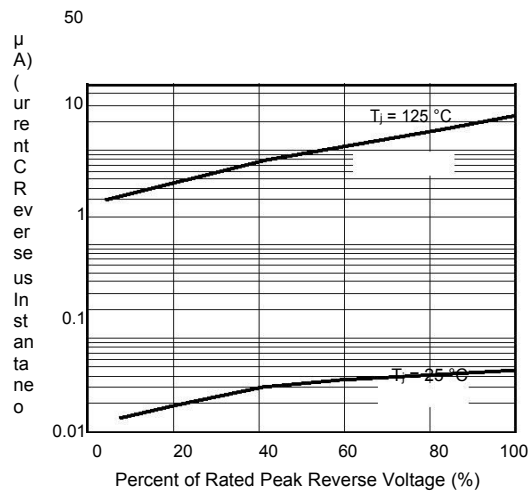
Figure 4. Typical Reverse Leakage Characteristics Per Diode
