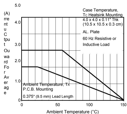
Figure 1. Derating Curve Output Rectified Current
