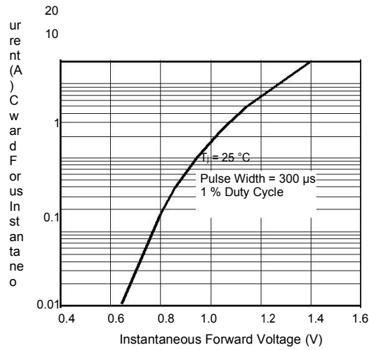
Figure 3. Typical Forward Characteristics Per Diode
