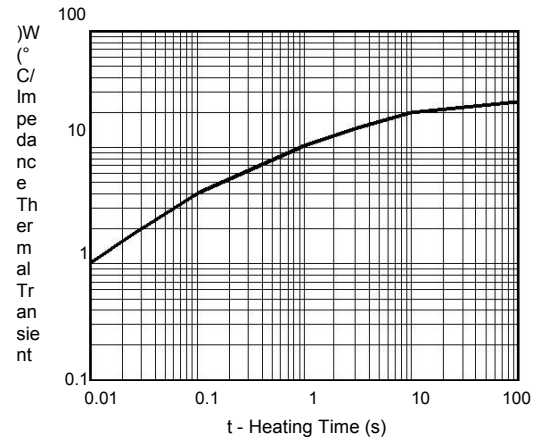
Figure 6. Typical Transient Thermal Impedance Per Diode
